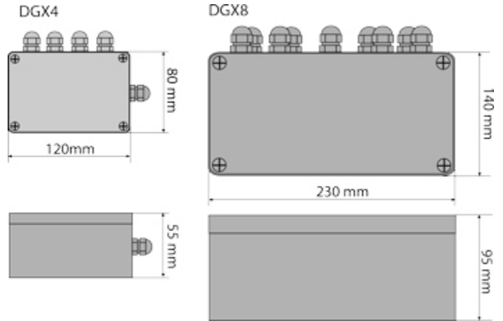
Conversion box, dimensions in mm.
